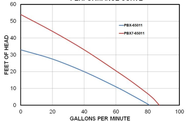
PERFORMANCE CURVE
