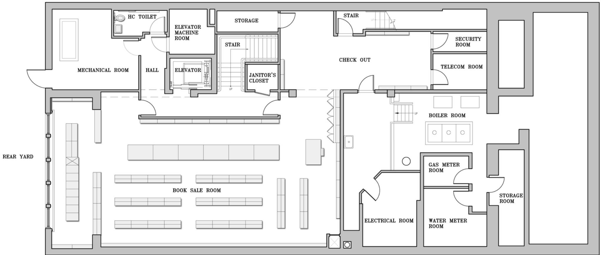
BASEMENT PLAN
